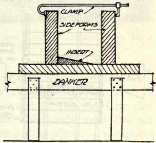
FIG. 35—SIMPLE WOOD MOLD—SECTION VIEW
